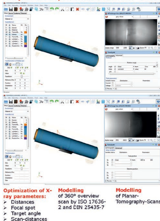
Fig. 15. aRTist scenarios designed for automated weld inspection with 360° circumferential scan (top) and Planar Tomographic scan (bottom) with modelled projections [18]
