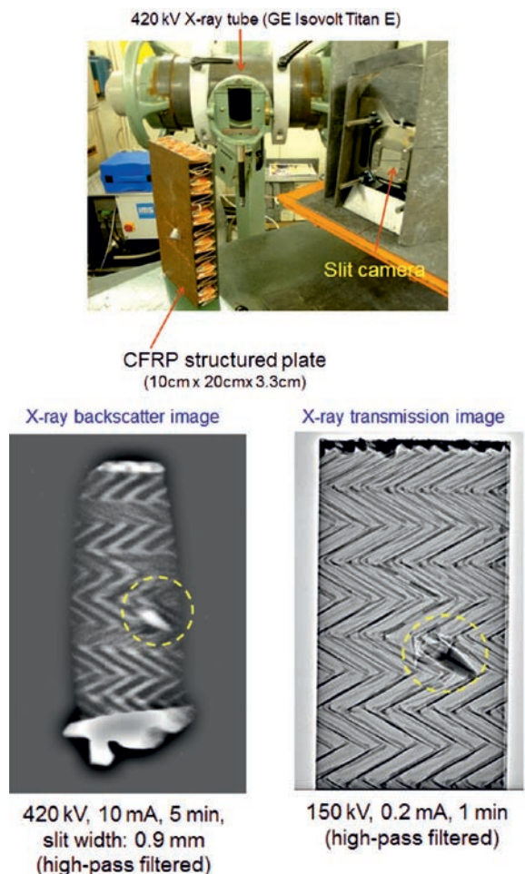
Fig. 12. Set up of a back scatter measurements of a CFRP structure (up) and back scatter image (left) in comparison to transmission radiograph (right) [35]
