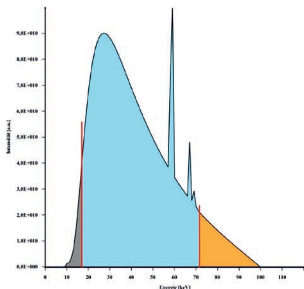
Fig. 7. Selective detection of a bremspectrum (example) by thresholding inside of the detector [2]
